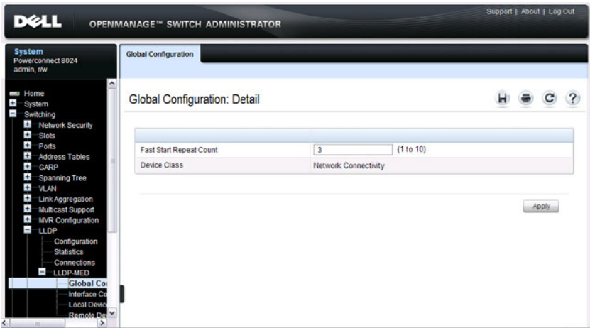
Figure 24-11. LLDP-MED Global Configuration
