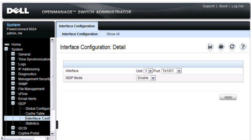
Figure 24-3. ISDP Interface Configuration
