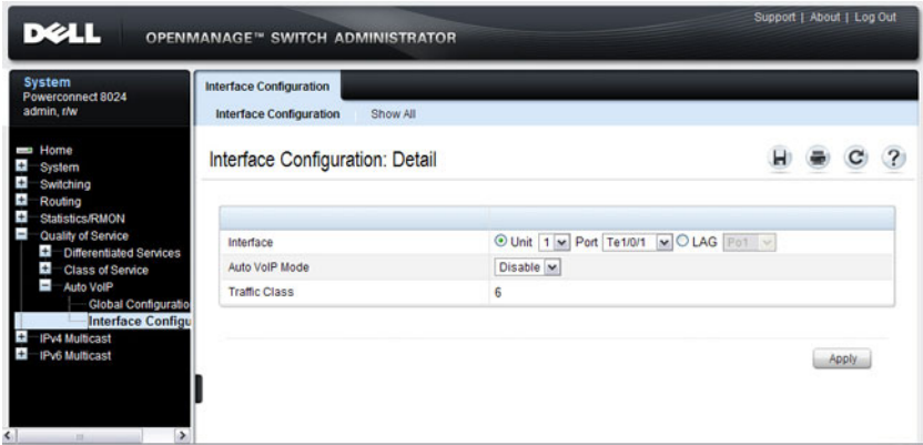
Figure 42-2. Auto VoIP Interface Configuration
