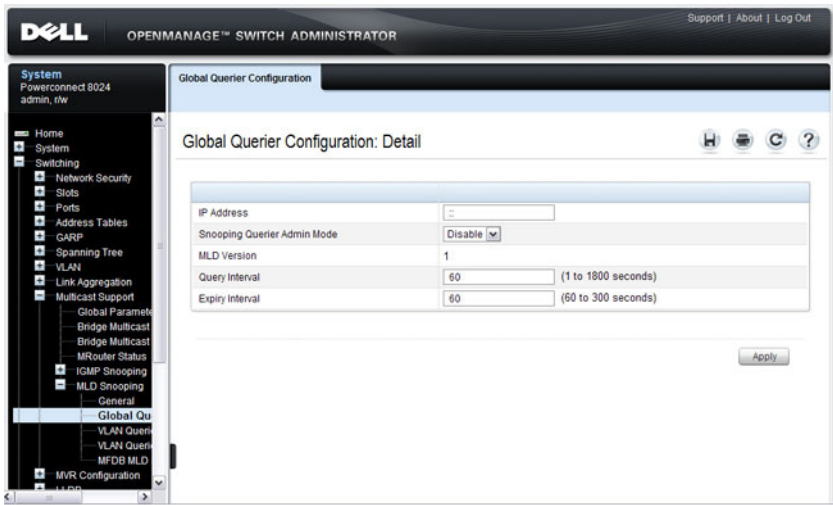
Figure 26-16. MLD Snooping Global Querier Configuration
