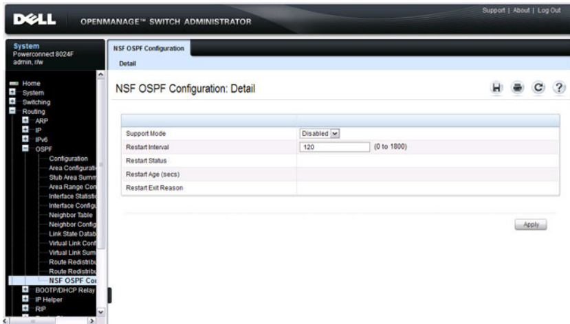
Figure 35-17. NSF OSPF Configuration
