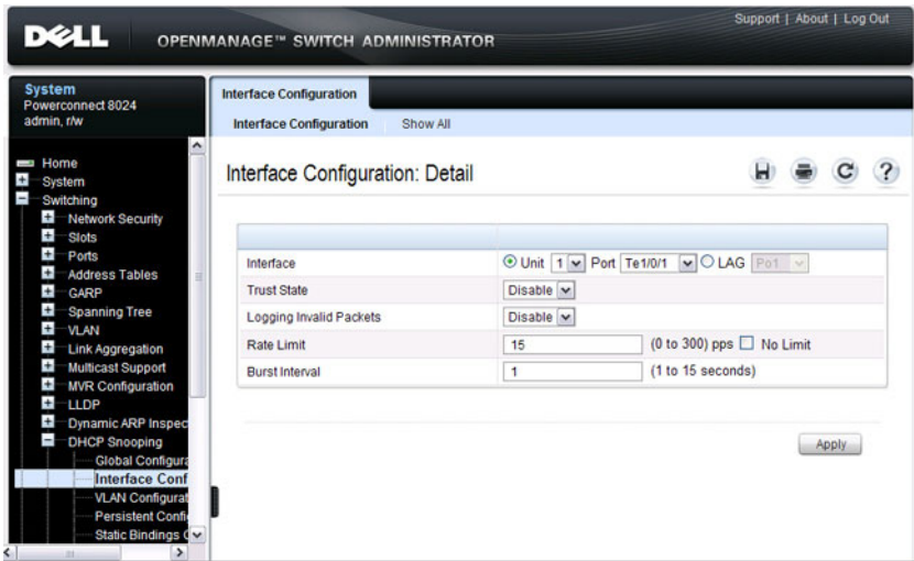
Figure 27-3. DHCP Snooping Interface Configuration
