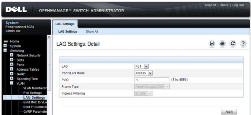
Figure 22-10. VLAN LAG Settings
