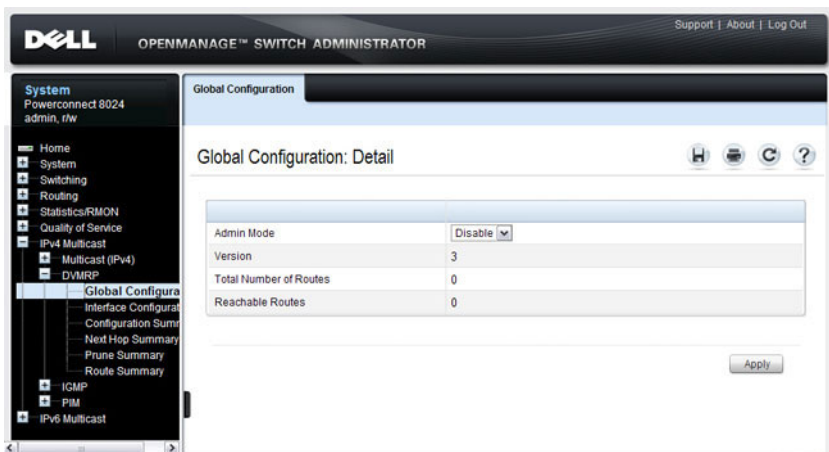
Figure 43-48. DVMRP Global Configuration
