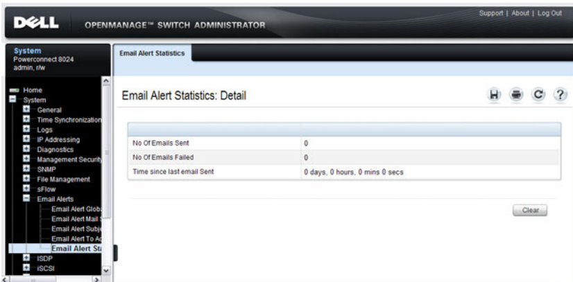
Figure 11-22. Email Alert Statistics
