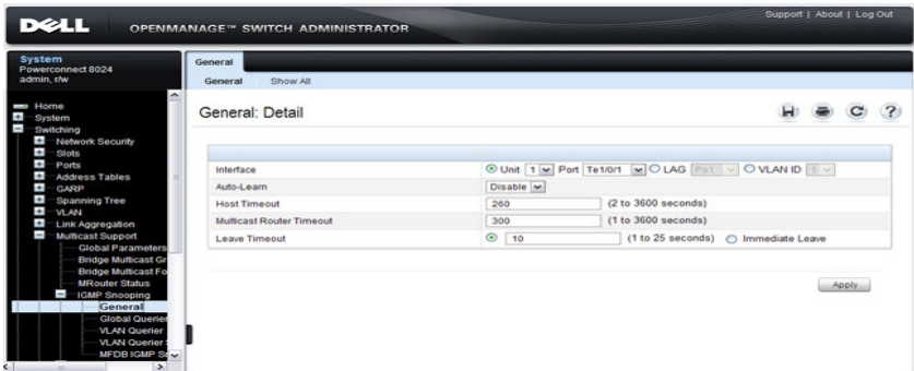
Figure 26-5. General IGMP Snooping
