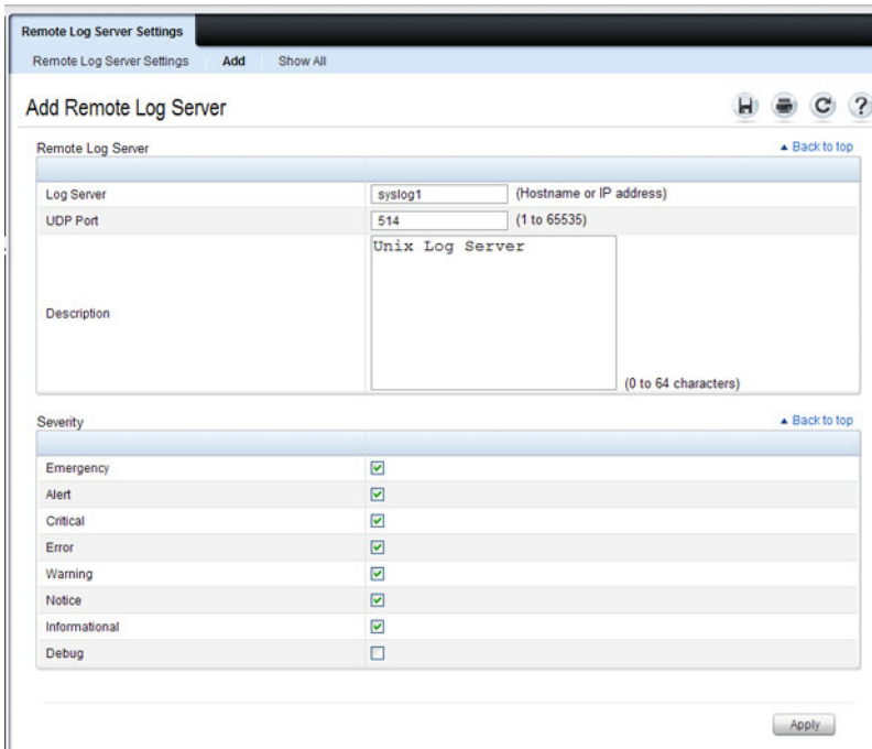
Figure 11-12. Add Remote Log Server
