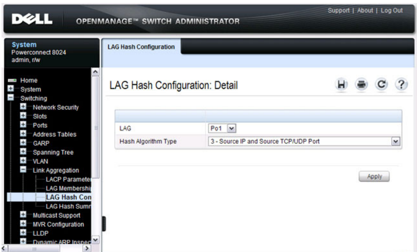
Figure 28-6. LAG Hash Configuration
