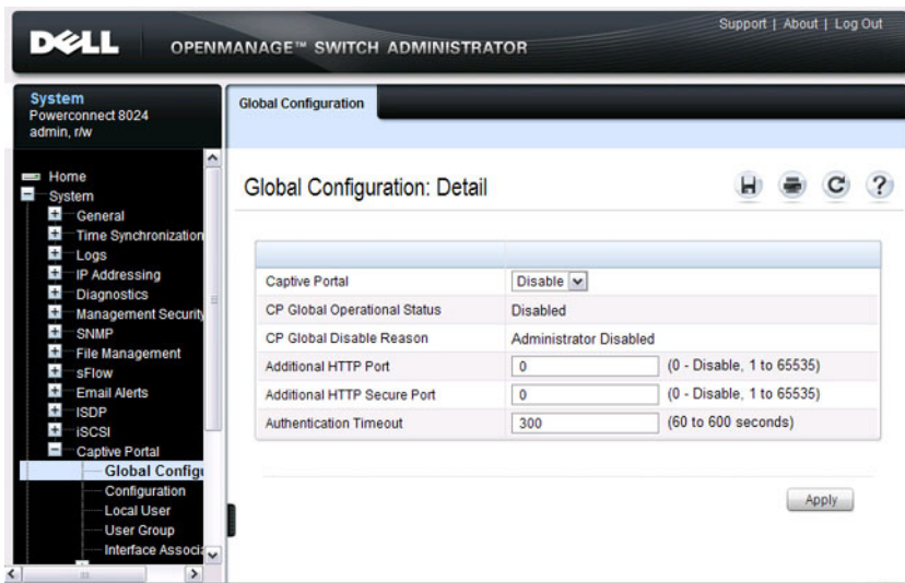
Figure 18-4. Captive Portal Global Configuration
