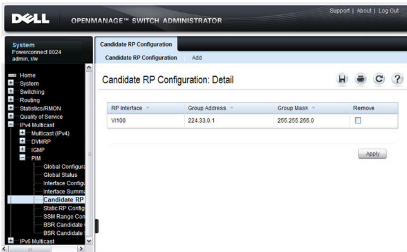
Figure 43-40. Candidate RP Configuration
