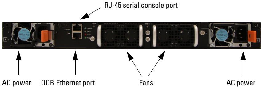
Figure 3-8. PowerConnect PC8100-Series Back Panel
