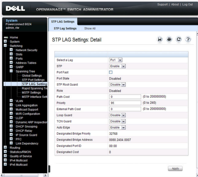
Figure 23-8. STP LAG Settings
