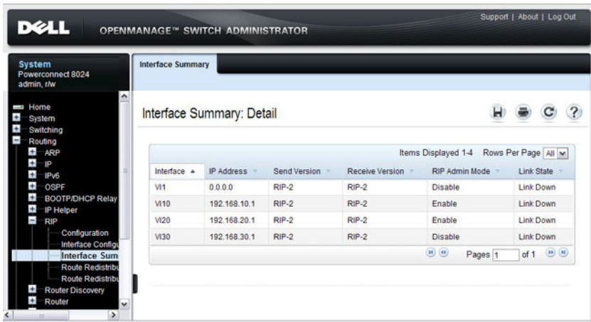
Figure 36-3. RIP Interface Summary
