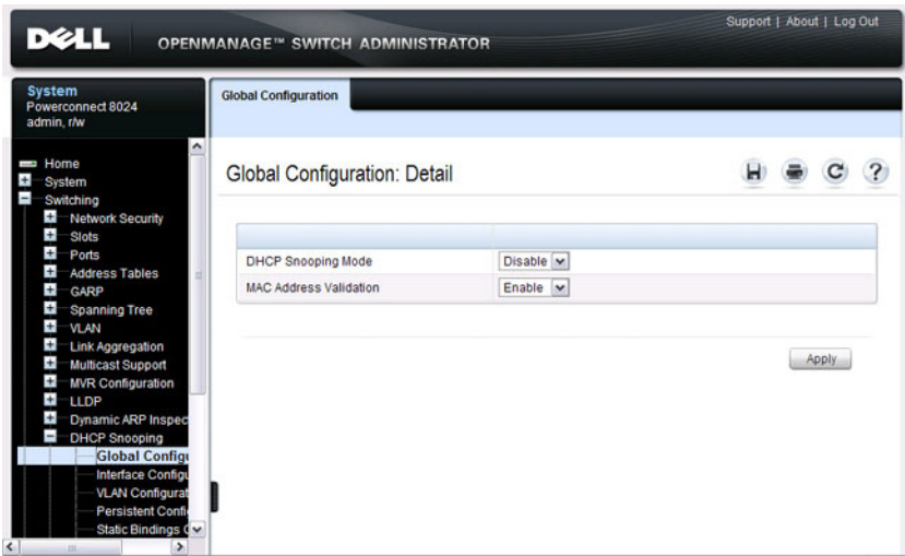
Figure 27-2. DHCP Snooping Configuration
