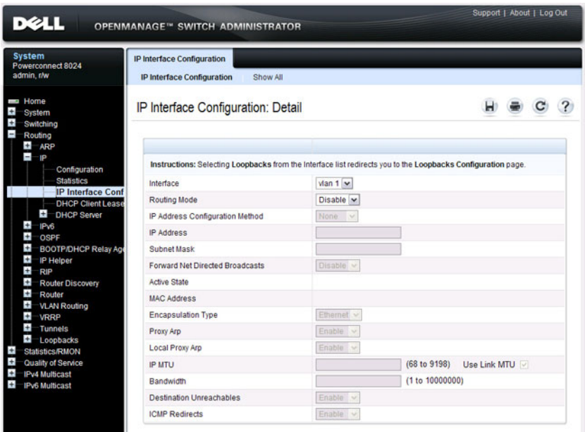
Figure 31-2. IP Interface Configuration
