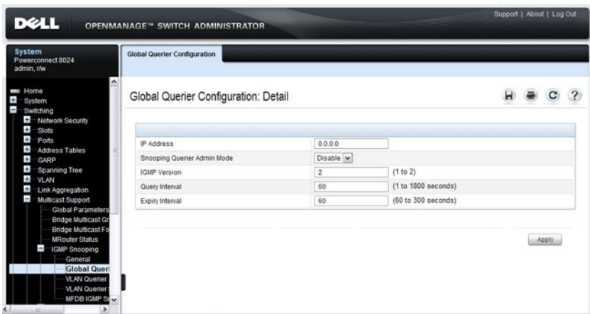
Figure 26-8. Global Querier Configuration
