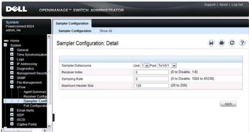
Figure 16-4. sFlow Sampler Configuration
