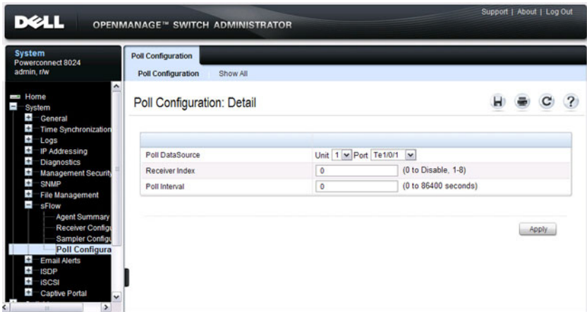
Figure 16-5. sFlow Poll Configuration
