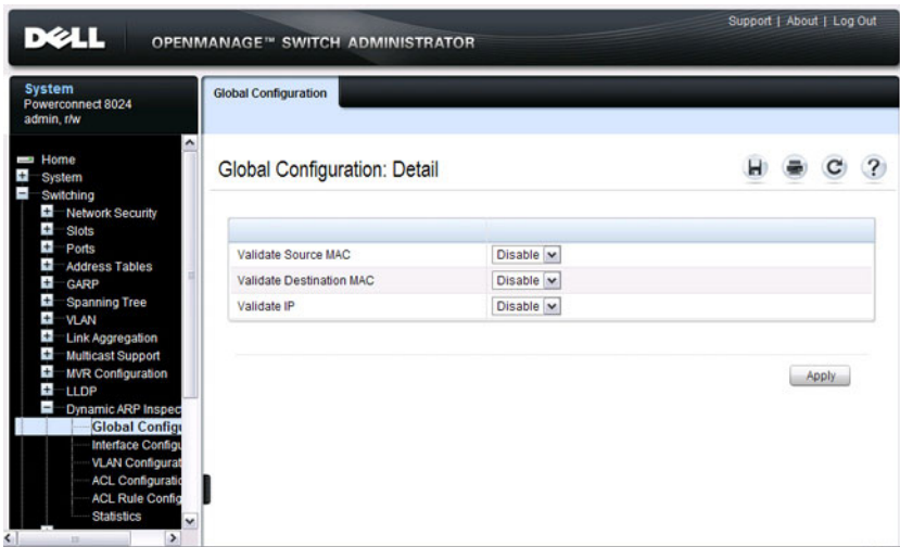
Figure 27-15. Dynamic ARP Inspection Global Configuration
