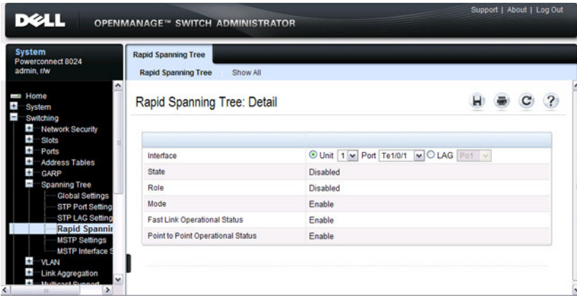
Figure 23-10. Rapid Spanning Tree
