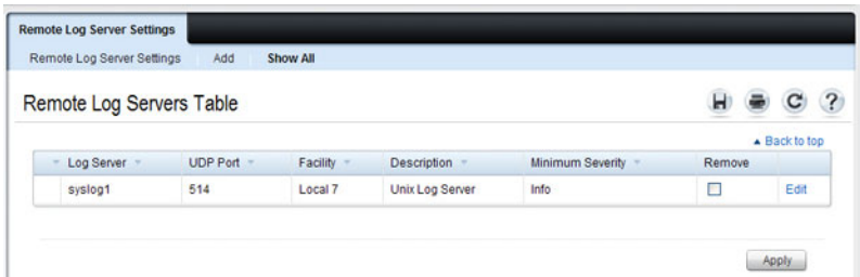
Figure 11-13. Show All Log Servers
