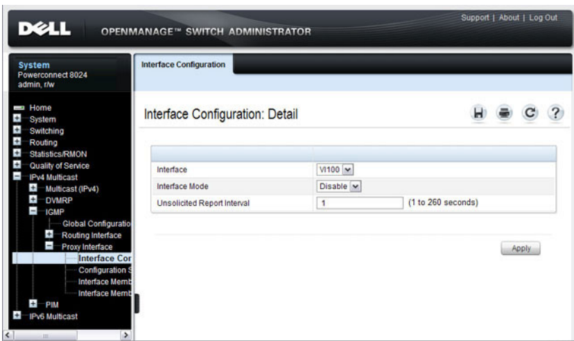
Figure 43-22. IGMP Proxy Interface Configuration
